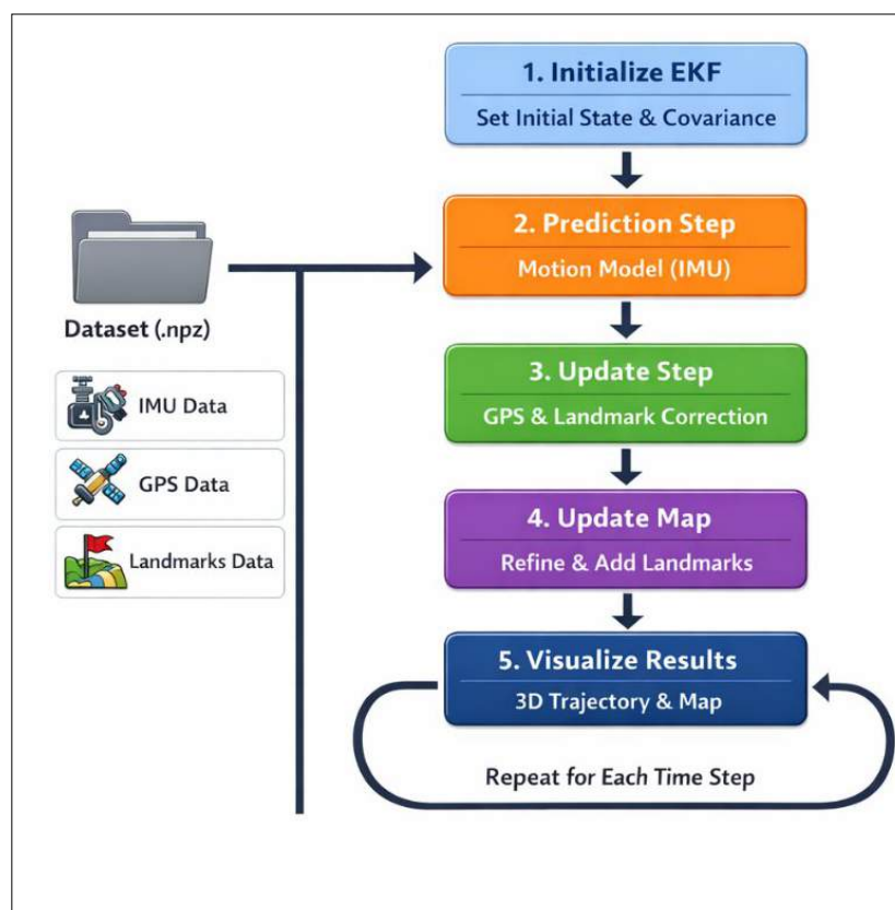
Fig:- Algorithm Flow of 3D EKF-SLAM
