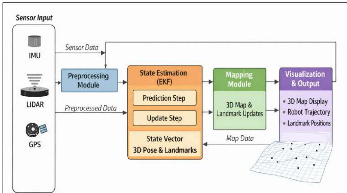
Fig:- System Architecture of 3D EKF-SLAM
