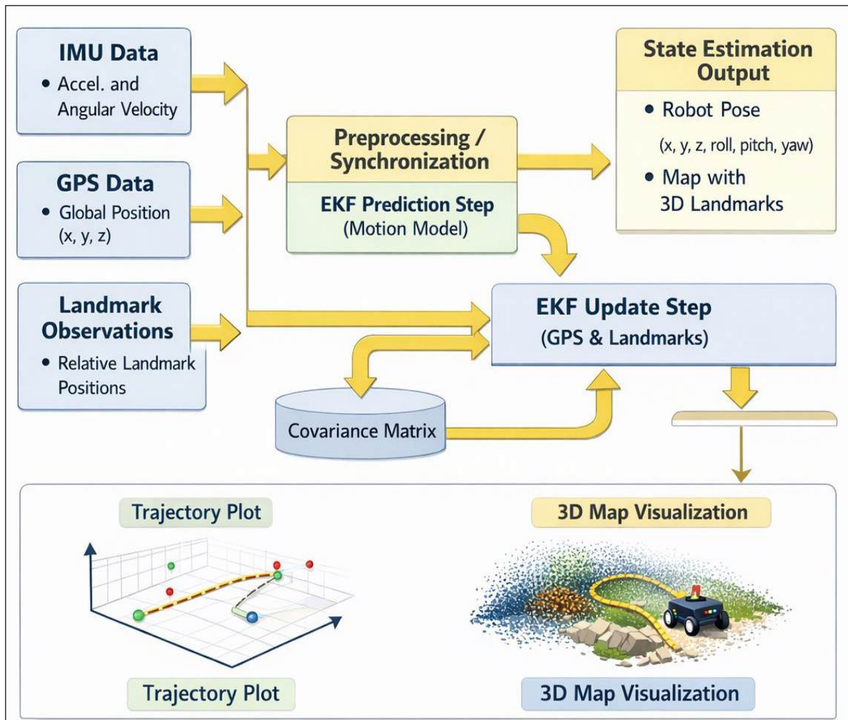
Fig:- 3D EKF-SLAM
